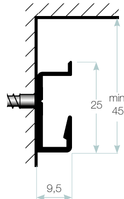
Rail 2842 - 25x9,5 mm
