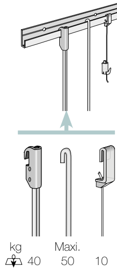
Rail 2840 - 27x10 mm
