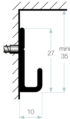
Rail 2840 - 27x10 mm
