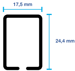
Rail 100 - 24x16 mm
