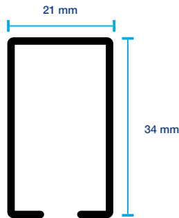
Rail 700 - 35x20 mm
