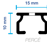
Rail 200 - 15x10 mm
