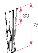
AGRAFE 4 BROCHES , acier zingué fil \varnothing 2 mm.
