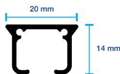
Rail KS - 20x14 mm
