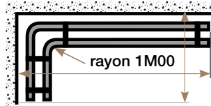
1 coude
